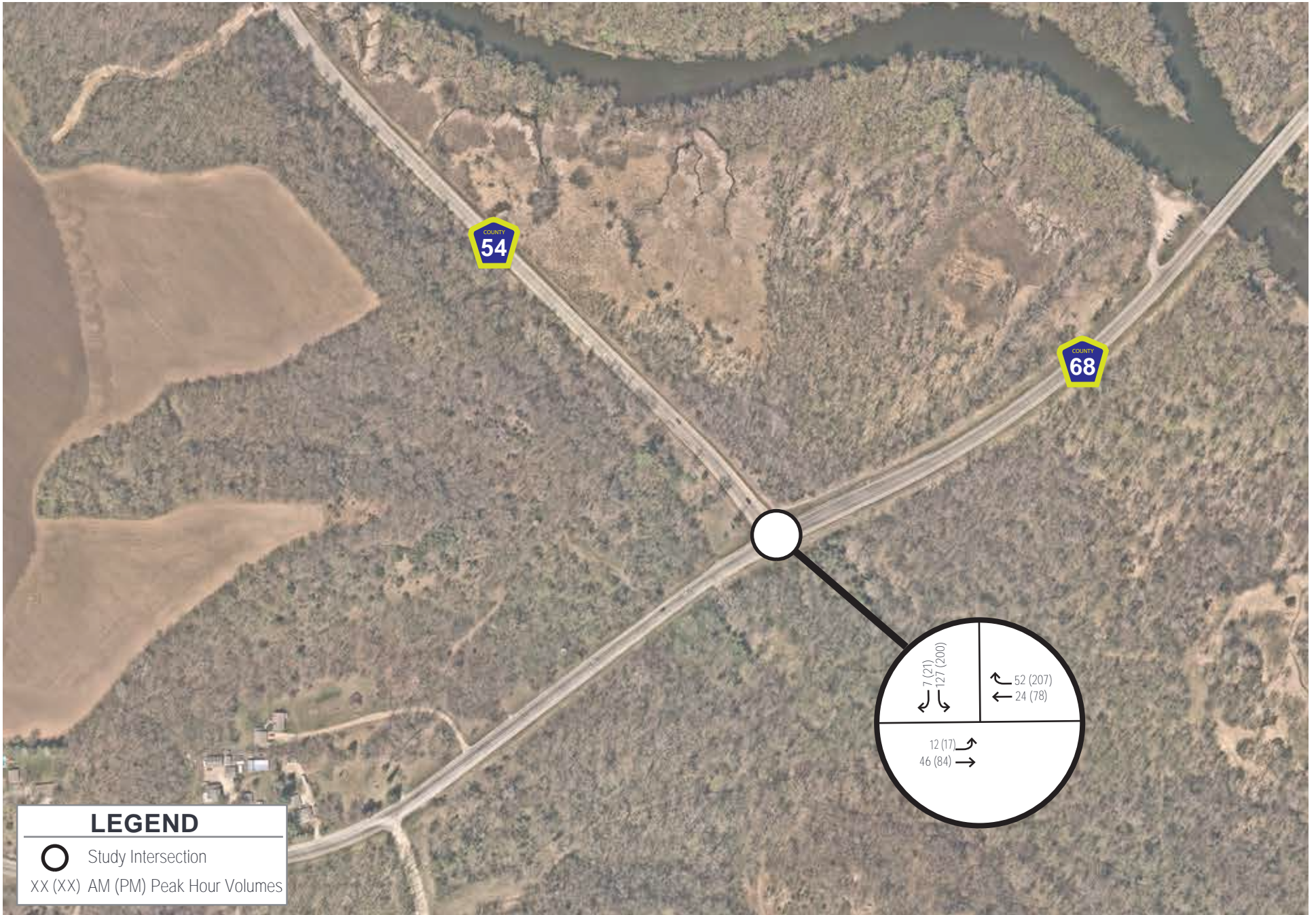
EXHIBIT 4 FUTURE YEAR 2040 PEAK HOUR TRAFFIC VOLUMES
